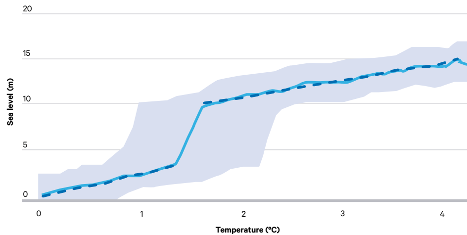
Figure 17. Committed sea level rise as a function of long-term global temperature increase
