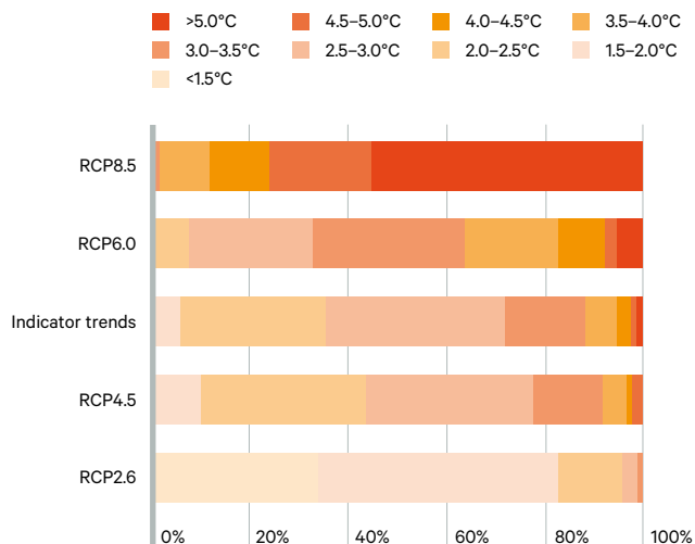
Figure 1b. Warming probability in different scenarios, in 2100
