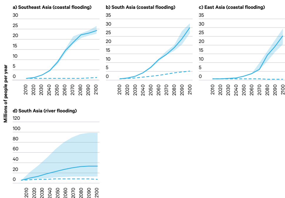
Figure 18. Populations in selected regions likely to experience coastal and river flooding
