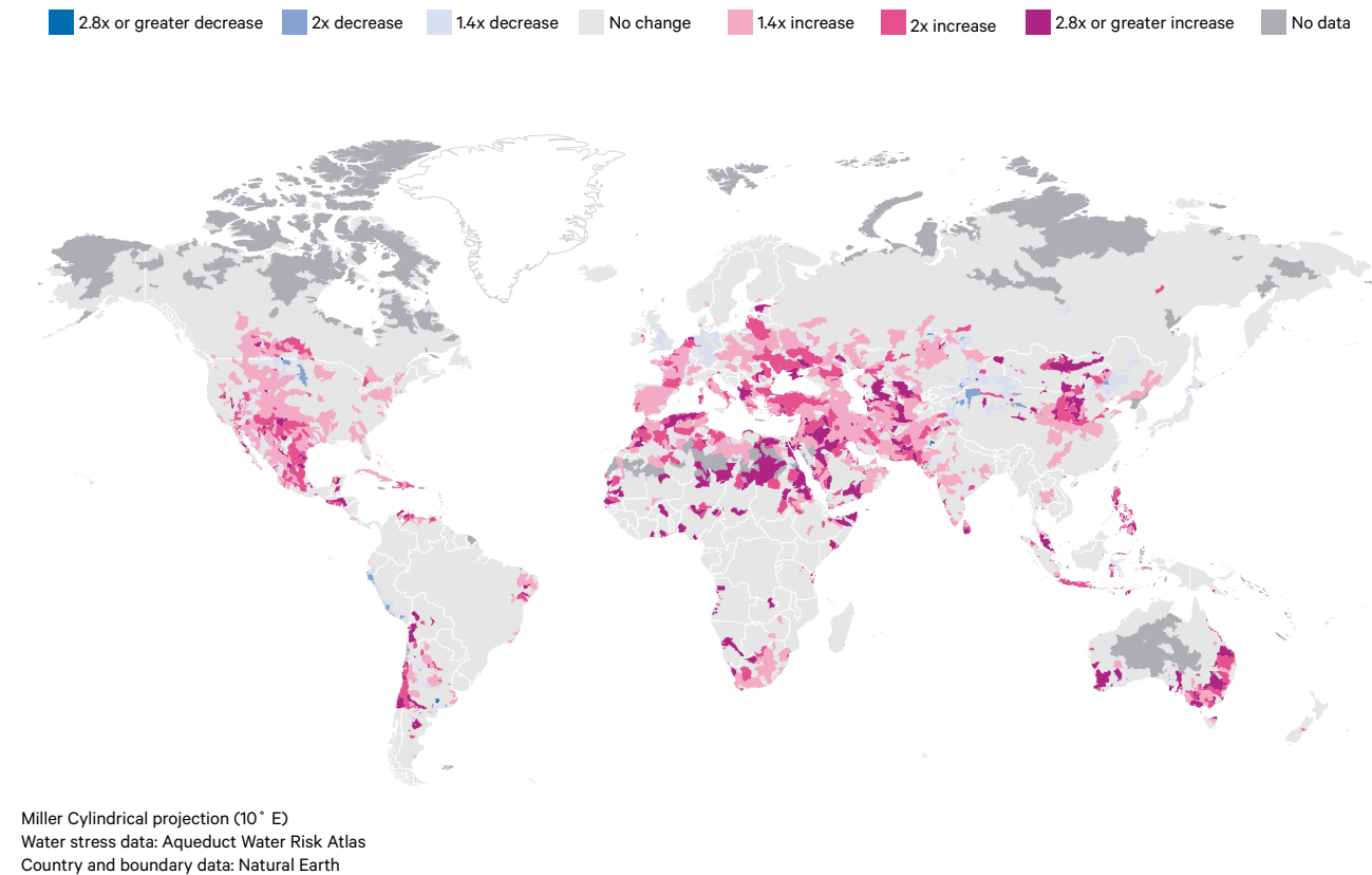
Figure 16. Regions of increasing water stress (demand relative to supply) in 2040, relative to 2019
