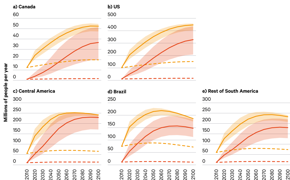
Figure 8. Populations within North, Central and South America experiencing heatwaves and major heatwaves
