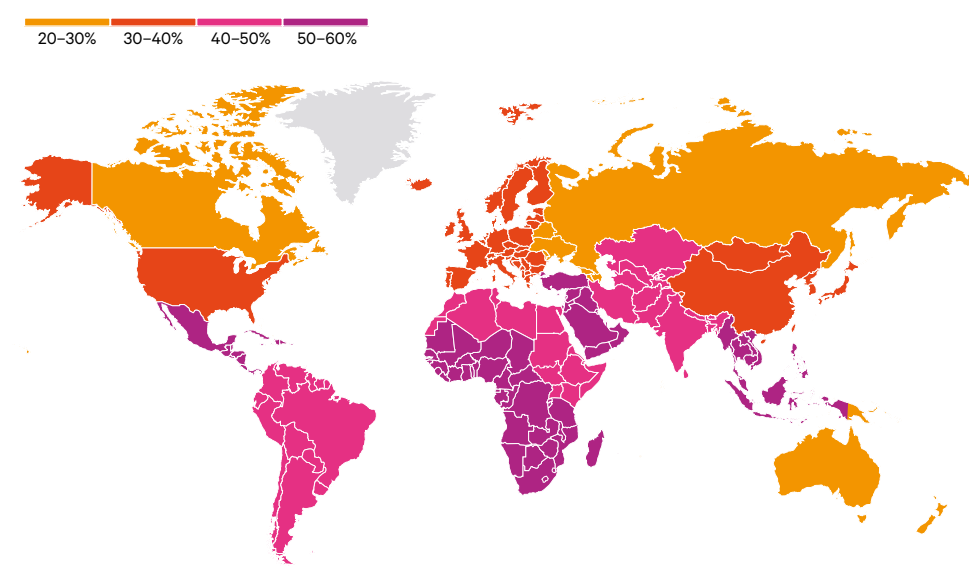
Figure 4. Proportion of regional populations experiencing major heatwaves, in 2040
