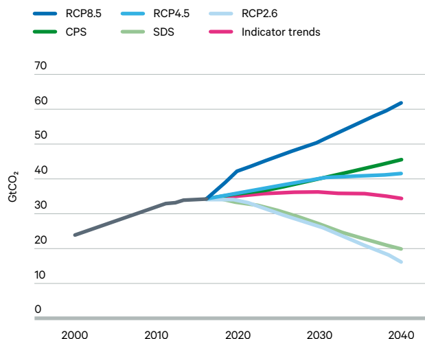
Figure 1a. Energy sector and industrial process CO 2 emissions to 2040, based on indicator trends
