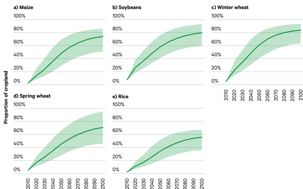
Figure 11. Proportion of global crop areas with reductions in crop duration periods of at least 10 days, by crop type
